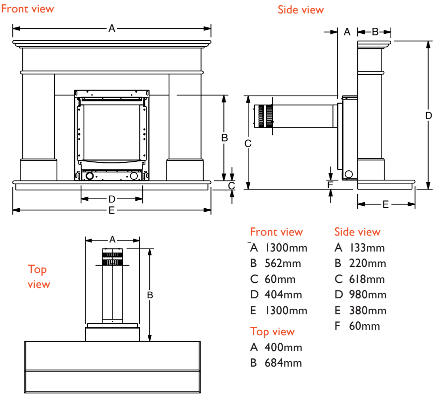
PASSION BALANCED FLUE
