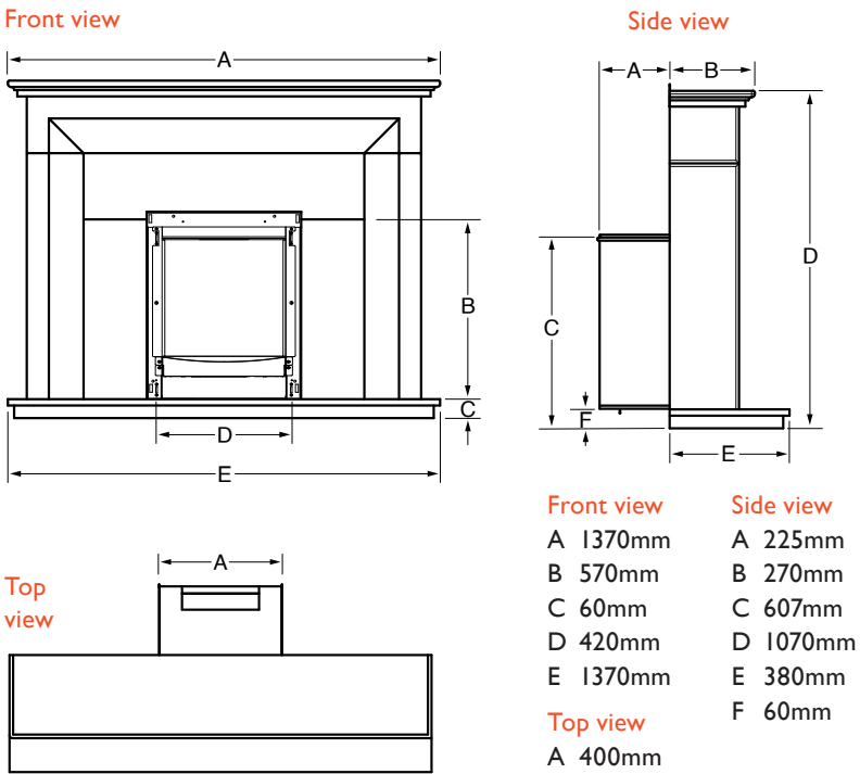
PASSION HE CONVENTIONAL FLUE
