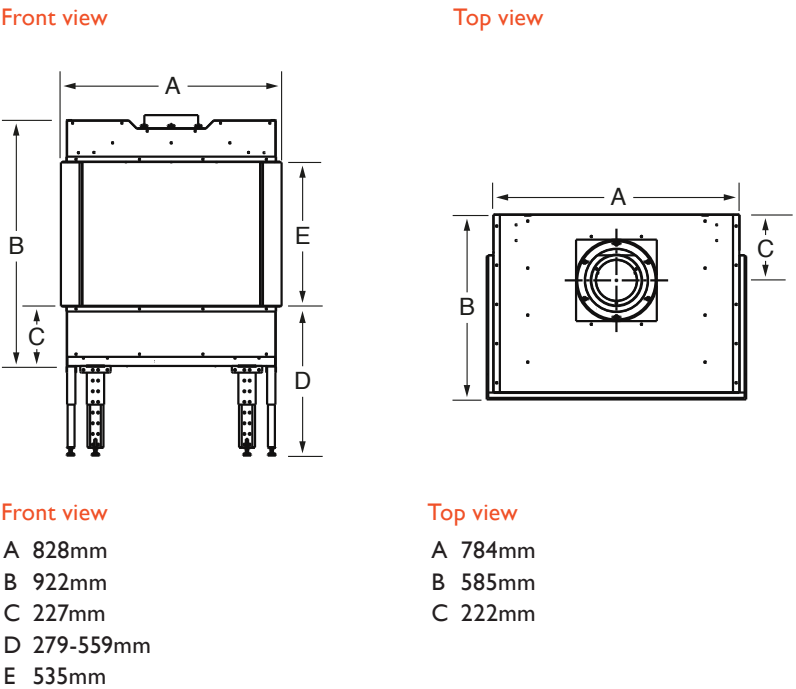
PASSION BALANCED FLUE
