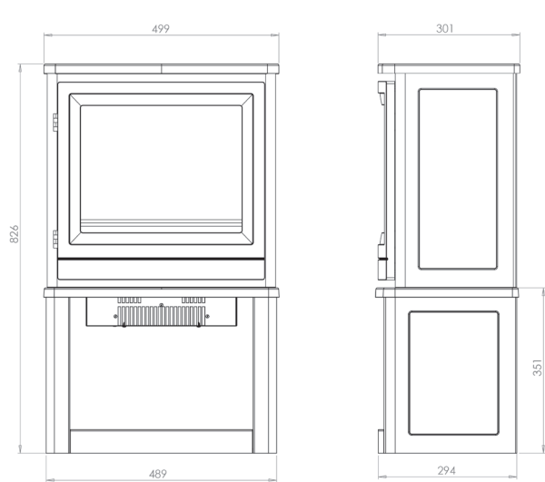
Horizon Stove with Log Store
